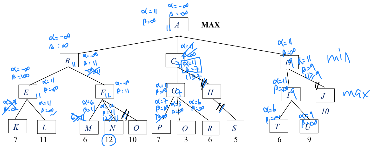
Figure 3: Game tree using Alpha-beta Pruning
